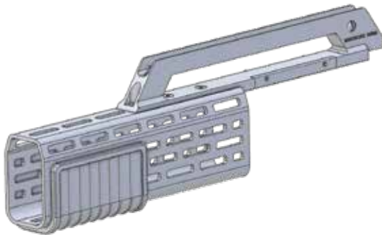
FIG. 4A: LEFT FRONT VIEW OF MA-38800 RIPLEY RAIL
