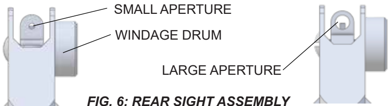
FIG. 6: REAR SIGHT ASSEMBLY
