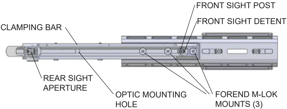
FIG. 2: TOP VIEW
